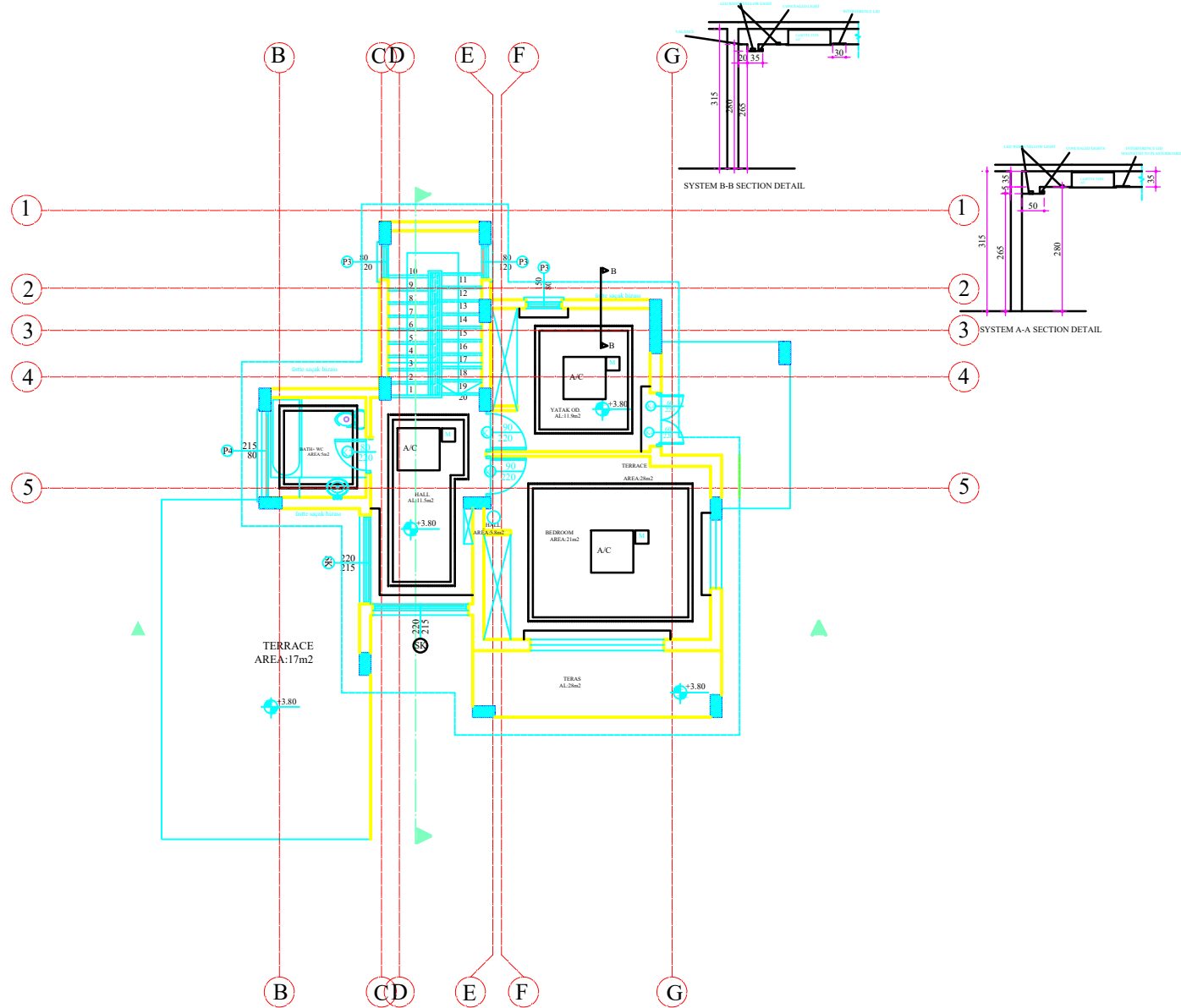
I. FLOOR PLAN SCALE:1/50 GROSS AREA:40m2
