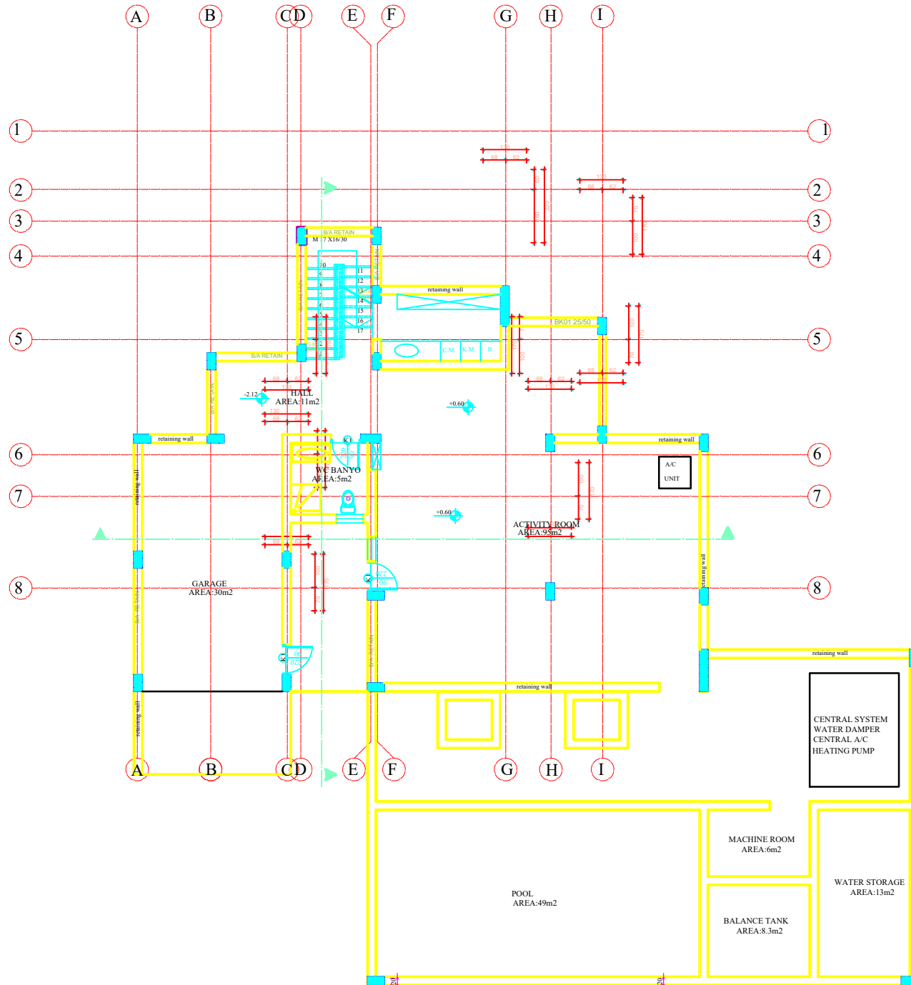
BASEMENT PLAN SCALE:1/50 GROSS AREA:62m 2
